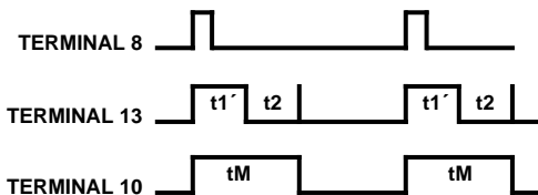
FIGURE 30. MONOSTABLE WAVEFORMS
